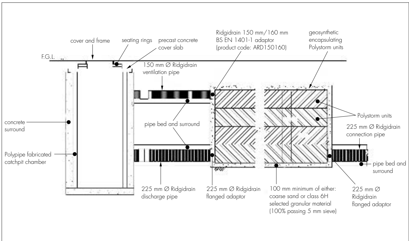
Figure 5 Typical Polystorm arrangement including ventilation pipe
