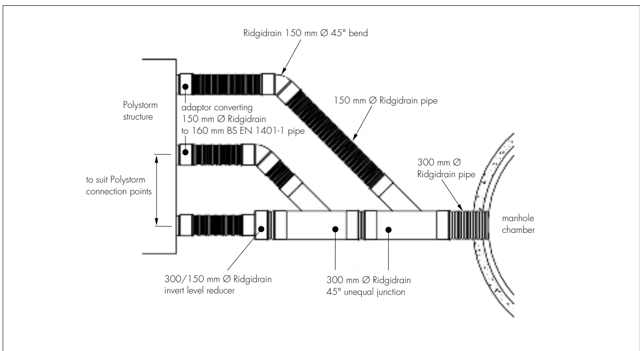
Figure 3 Typical manifold design
